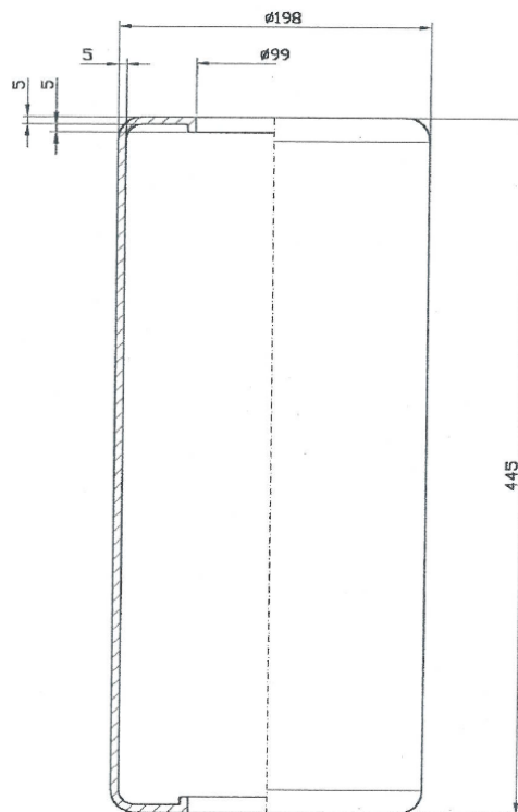
Diagram For 40 Liter Bladder
