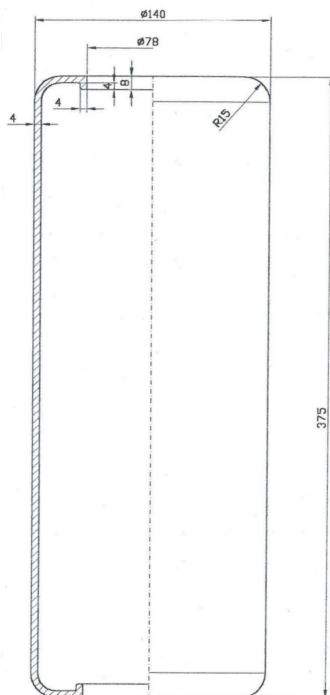
Diagram For 20 Liter Bladder
