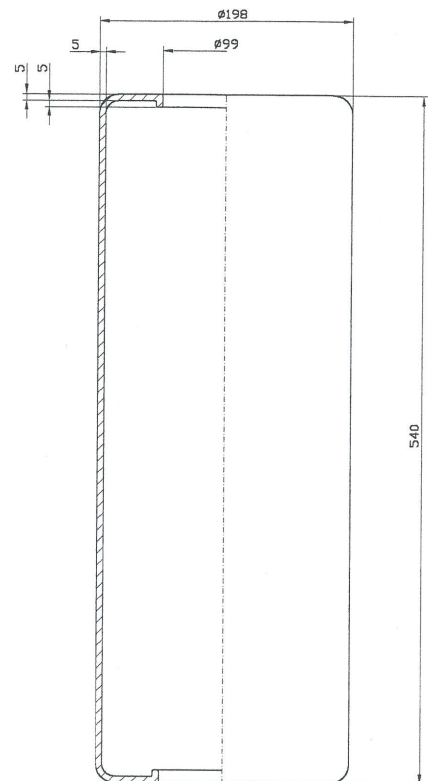
Diagram For 80 Liter Bladder
