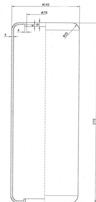
Diagram For 20 Liter Bladder
