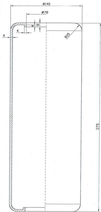
Diagram For 20 Liter Bladder
