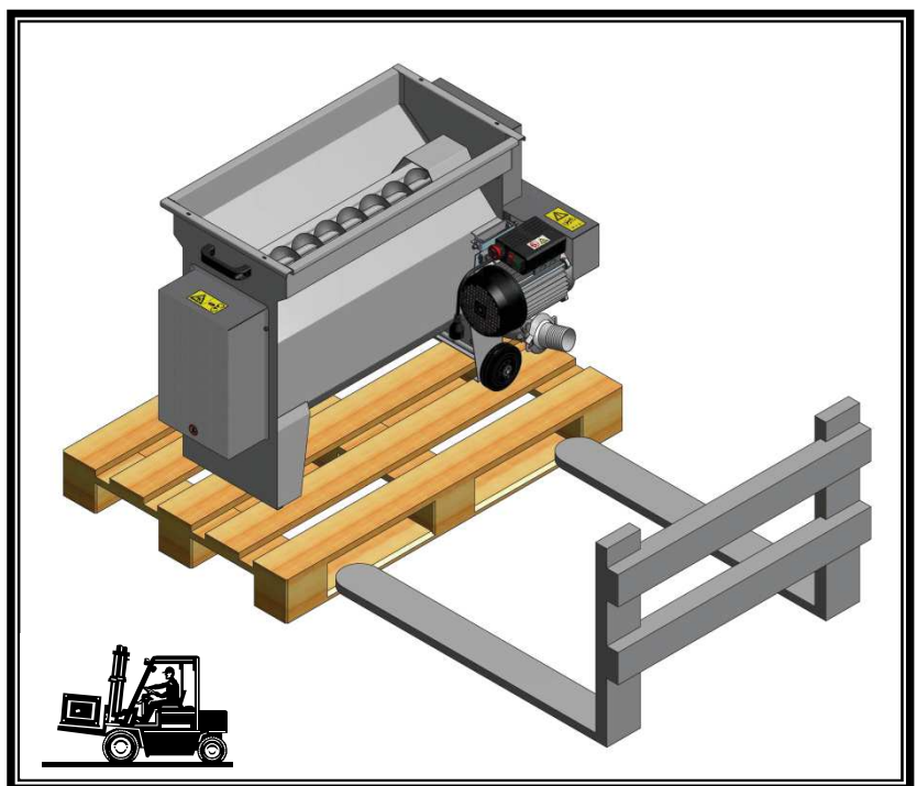
Fig. 3.2 Transport and lifting
