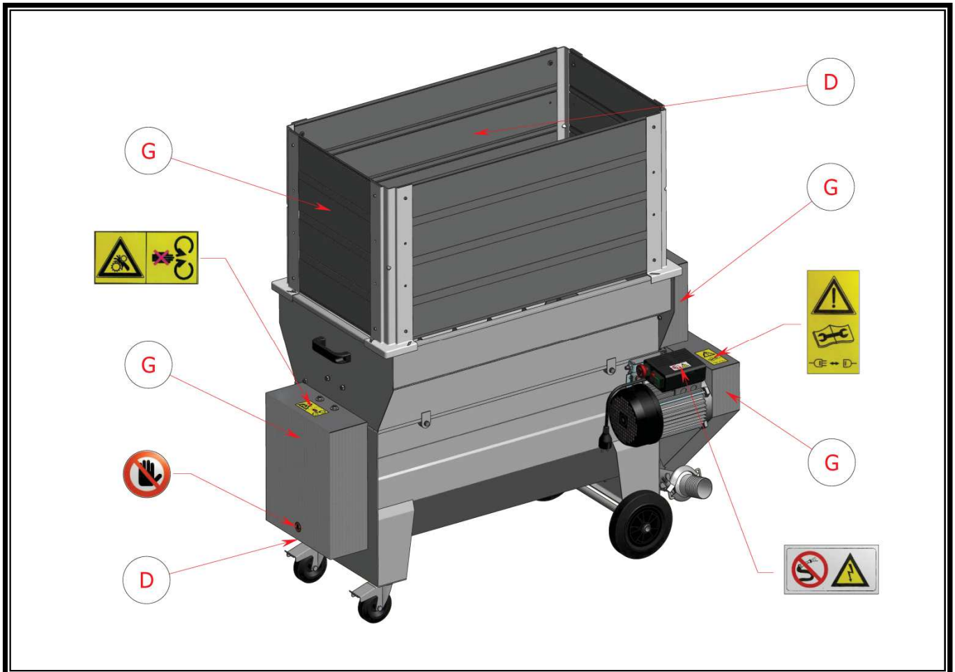
Fig. 4. D: areas of danger G: fixed guards
